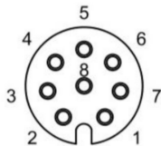
Face View M12 Female
