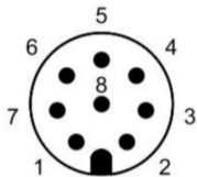
Face View M12 Male
