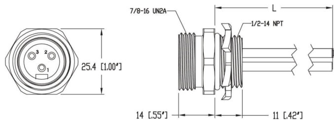
RSFPA 3-1/2NPT-802/xM
