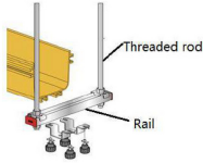
SUPPORTING—THREADED ROD SUSPENSION
