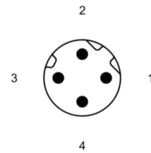
Technical Data Side 2 M12 Male
