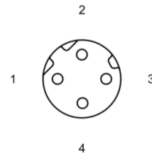
Technical Data Side 2 M12 Female
