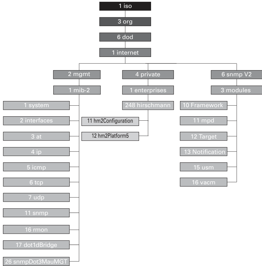
Figure 132: Tree structure of the Hirschmann MIB
