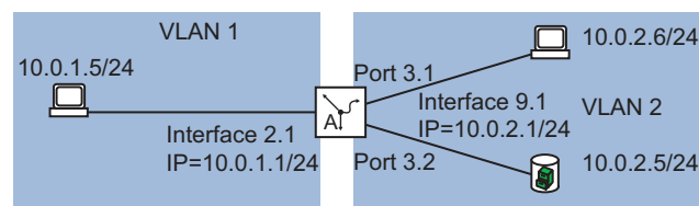
Figure 76: VLAN-based router interface
