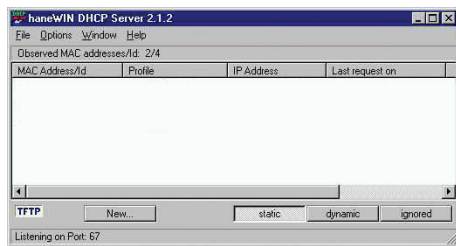
Figure 124: Start window of the haneWIN DHCP Server program
