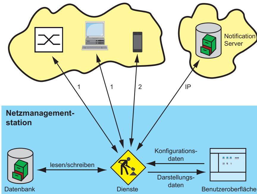
Abb. 1: Architektur 1 - SNMP-Get/Set/Trap, HiDiscovery, Ethernet/IP, Modbus/TCP, Ping, http, https, 2 - http, https
