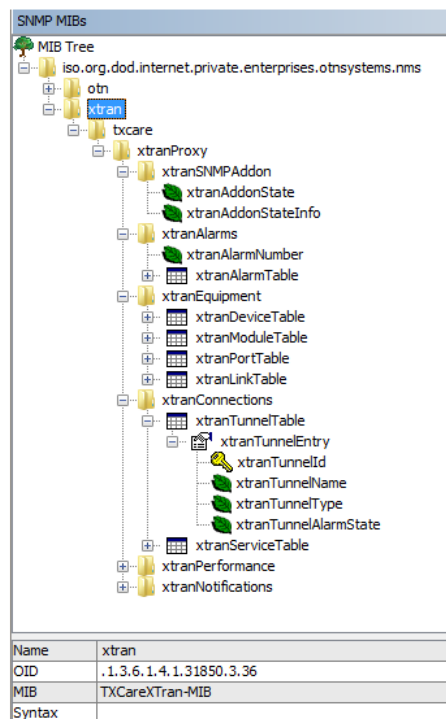
Figure 5 HiProvision MIB Window
