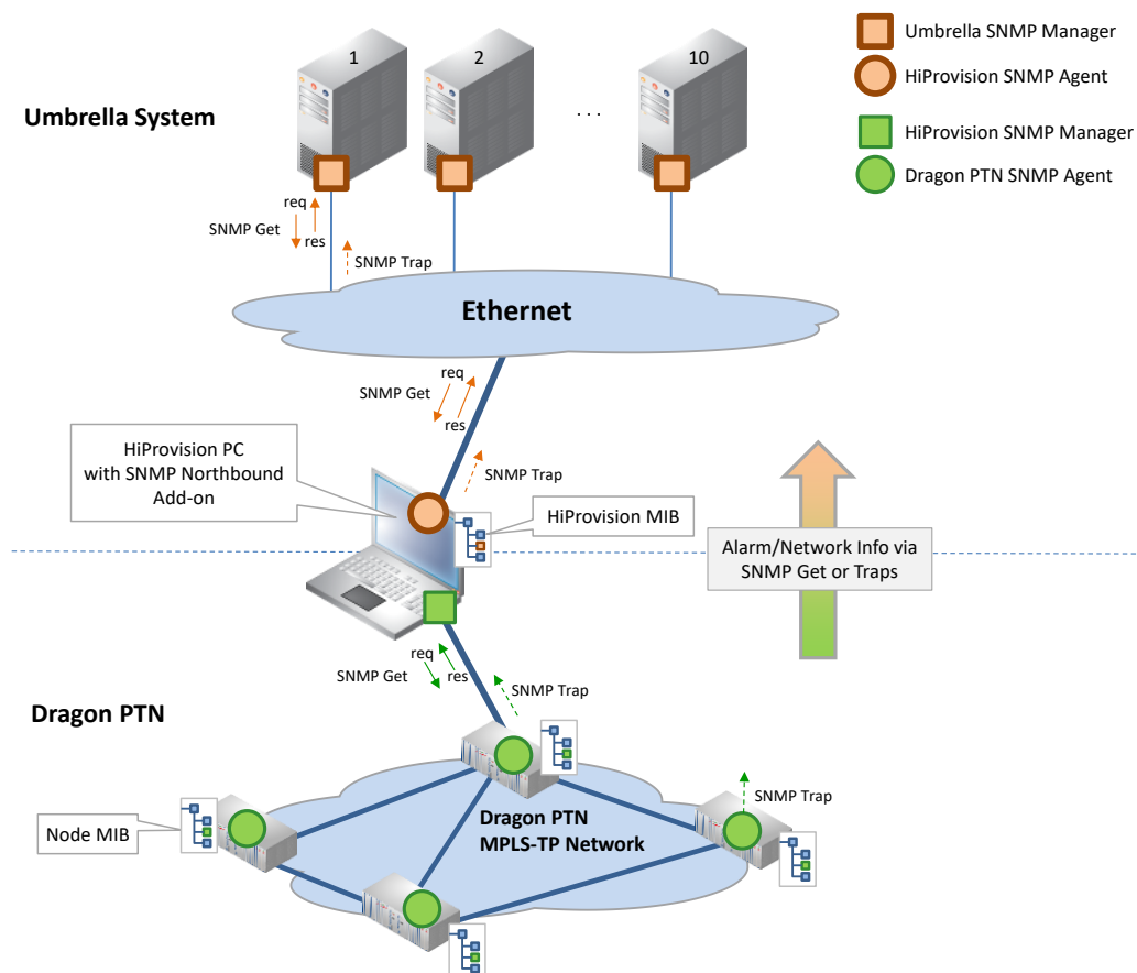
Figure 1 SNMP Northbound Example
