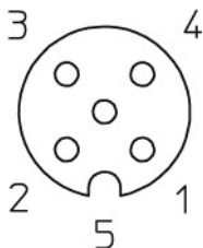
Figure 6: Schematic drawing, port X1 to X8
