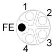
Figure 5: Schematic diagram of the M12 L-coding (socket), port X04 (OUT)
