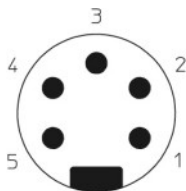
Figure 2: Schematic drawing, port X03 (IN)
