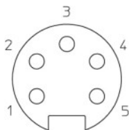
Figure 3: Schematic drawing, port X04 (OUT)
