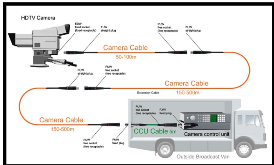
The lengths shown are examples. Cables are available in various lengths.
