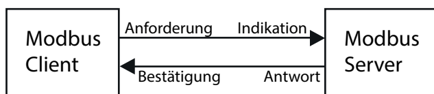
Abb. 66: Modbus TCP/IP Client/Server-Modus
