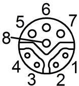
Figure 5: Schematic diagram of the M12 Hybrid (socket)
