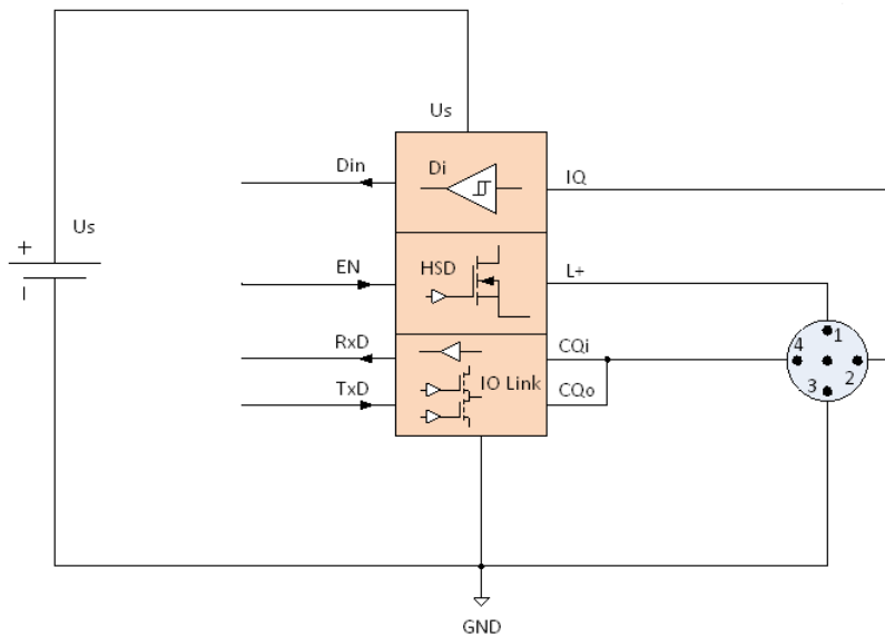
Figure 34: Block diagram Class-A Port
