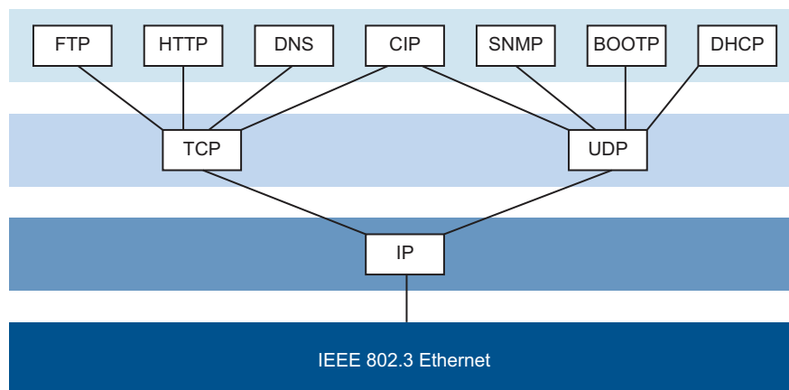
Abb. 59: IEEE802.3 EtherNet/IP
