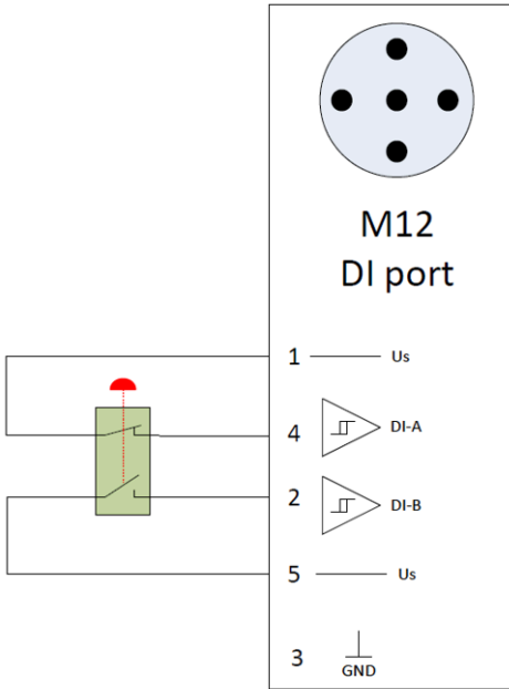
Figure 61: Internal F-DI block diagram
