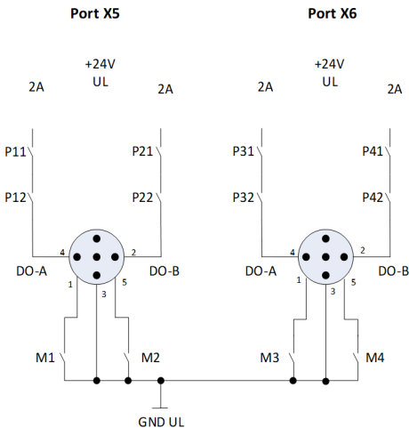
Figure 68: Schematic illustration of the DO functionality
