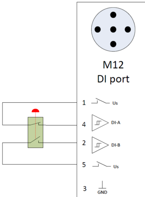
Figure 66: Internal F-DI block diagram
