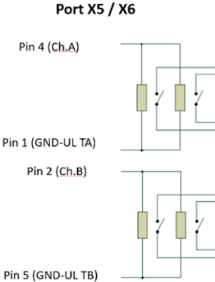
Figure 70: Schematic illustration with two redundant actuators
