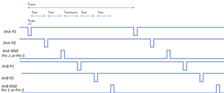
Figure 22: Diagram: F-DO test pulse timing
