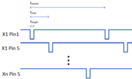
Figure 67: Diagramm: F-DI test pulse timing
