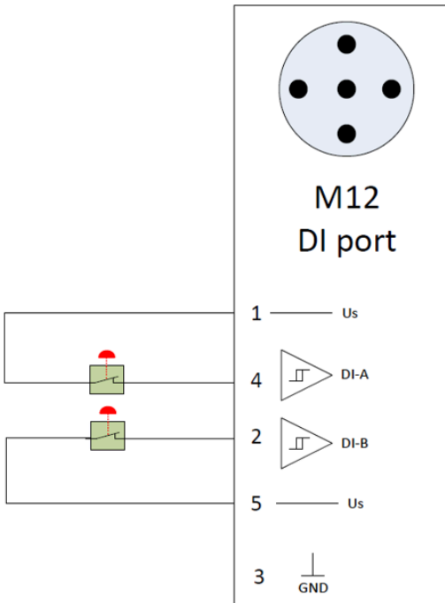
Figure 60: Internal F-DI block diagram
