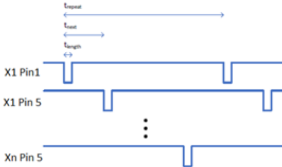
Figure 64: Diagramm: F-DI test pulse timing
