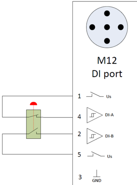
Figure 62: Internal F-DI block diagram
