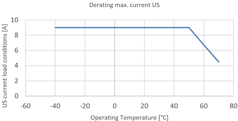
Figure 71: Derating of U S
