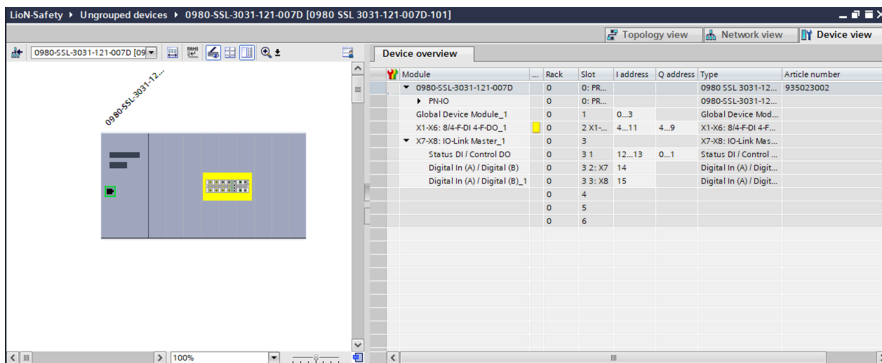
Figure 10: Device configuration
