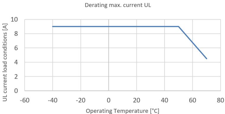
Figure 72: Derating of U_L
