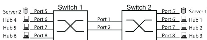
Abb. 41: Link Aggregation Switch-zu-Switch-Netz
