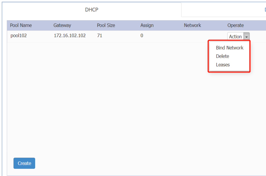
Figure 120: DHCP pool
