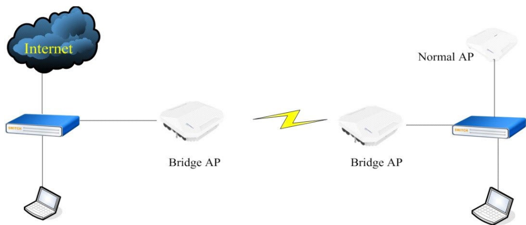
Figure 99: Bridge topology
