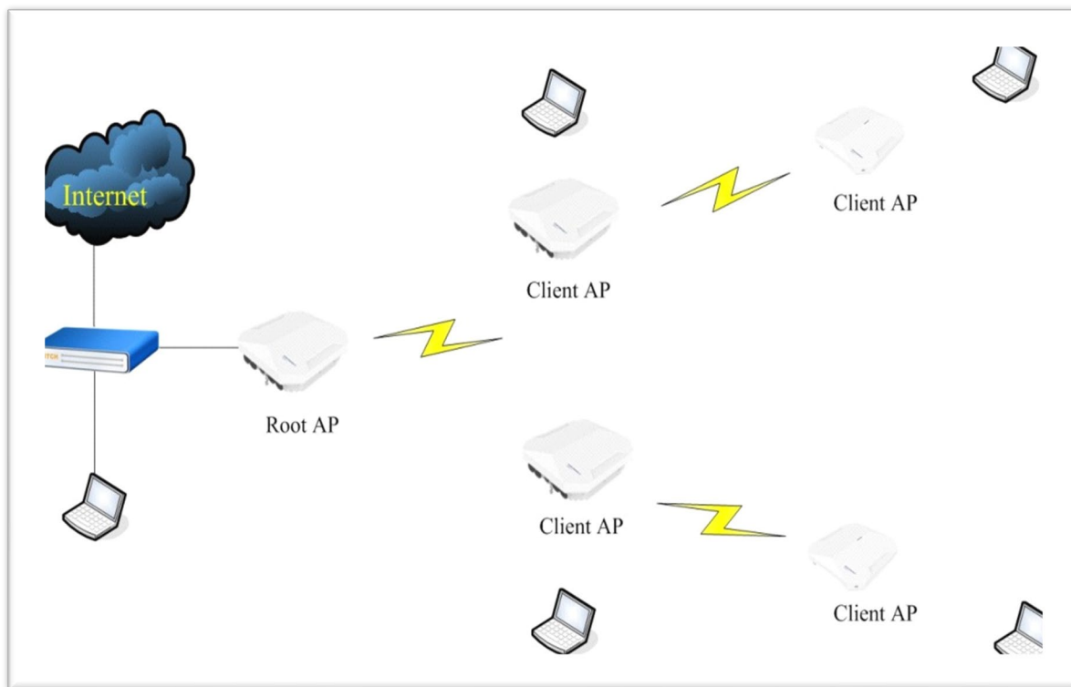
Figure 110: MESH topology
