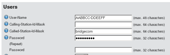
Figure 41: Creating a new user account using WEBconfig
