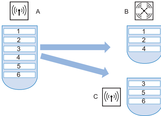
Figure 14: Split MAC in central WLAN management
