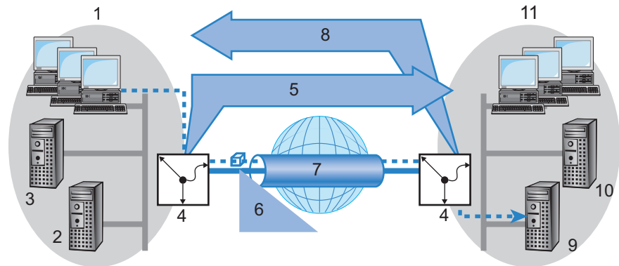
Figure 119: Network coupling
