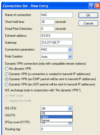
Figure 74: Editing an entry in the connection table
