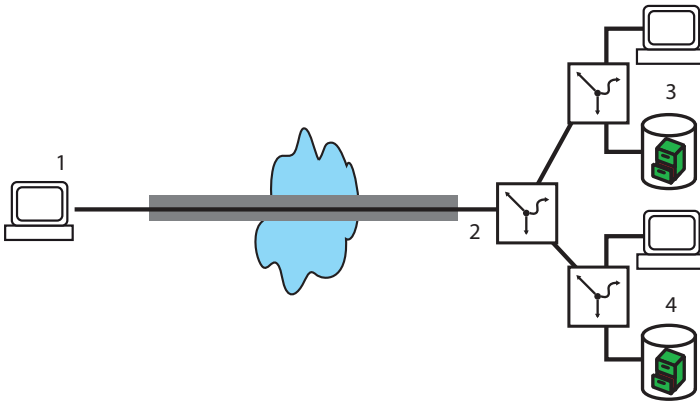
Figure 76: Various connected IP networks 1: Computer with remote access 2: IP network: 10.2.x.x 3: IP network: 192.x.x.x 4: IP network: 172.x.x.x
