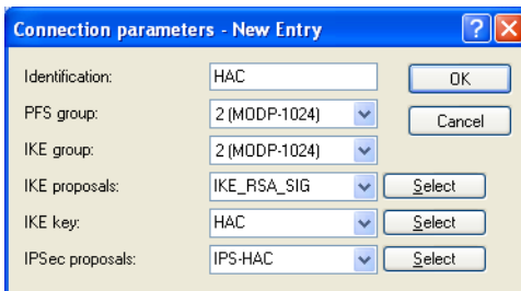
Figure 100: Checking the connection parameters in LANconfig
