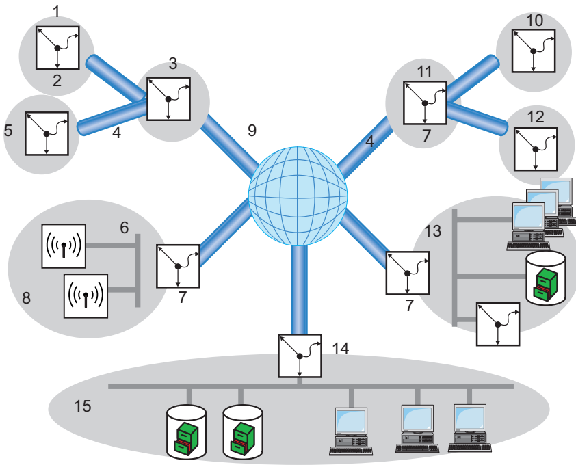
Figure 120: Centralized monitoring and control of networks for different clients
