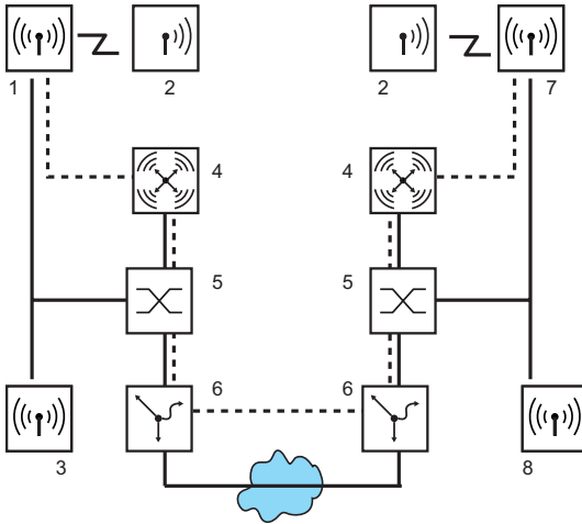
Figure 43: Overlay networks across several IP networks
