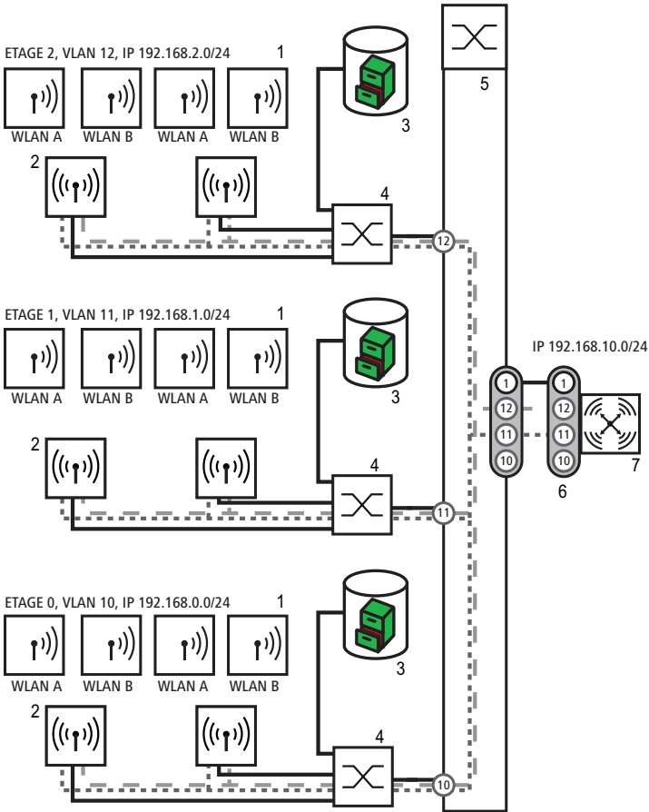
Figure 52: Application example for layer-3 roaming
