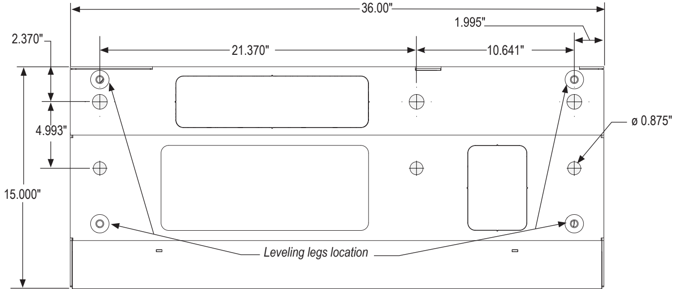
Bottom view of the cabinet
