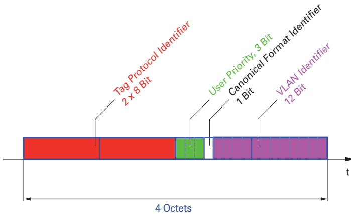
Figure 17: Structure of the VLAN tagging
