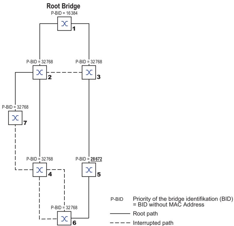
Figure 13: Example of manipulating the root path
