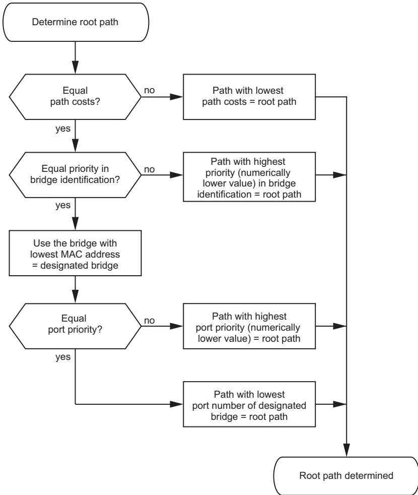
Figure 11: Flow chart for determining the root path
