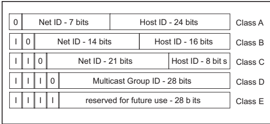
Figure 4: Bit representation of the IP address
