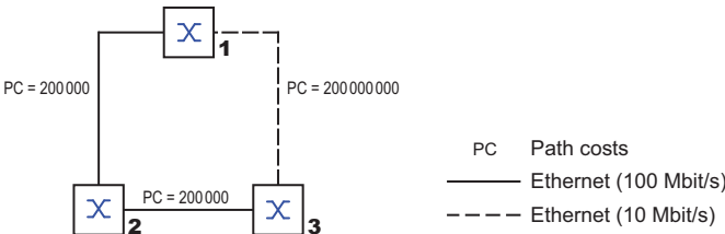
Figure 7: Path costs
