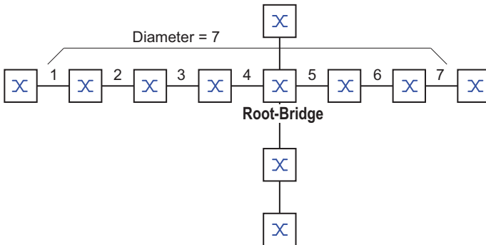
Figure 9: Definition of diameter
