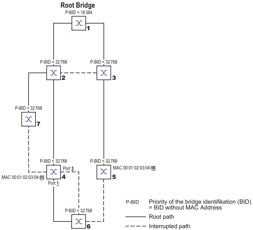
Figure 12: Example of determining the root path
