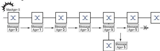
Figure 10: Transmission of an STP-BPDU depending on MaxAge
