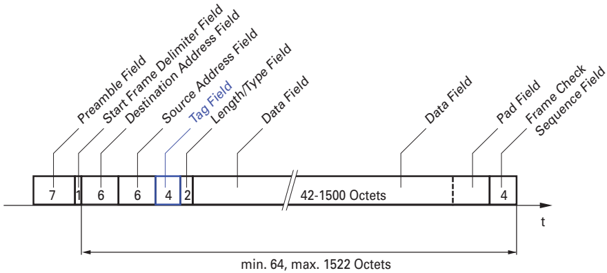
Figure 16: Ethernet data packet with tag
