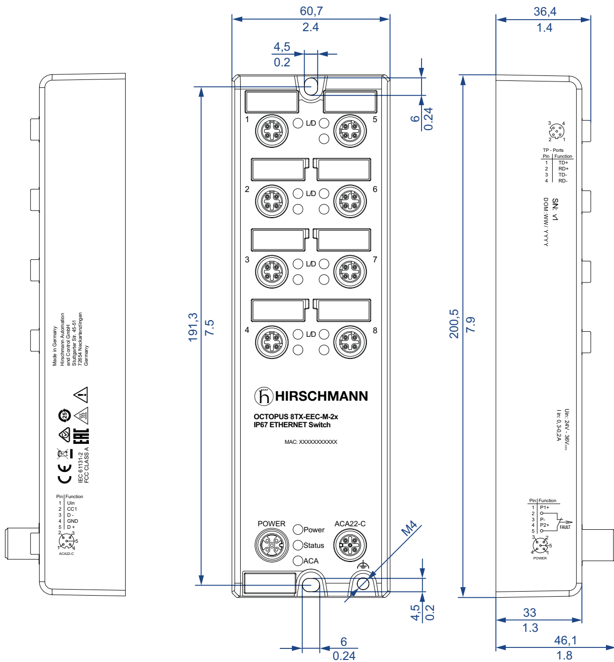
Figure 13: OCTOPUS 8TX-EEC-M
