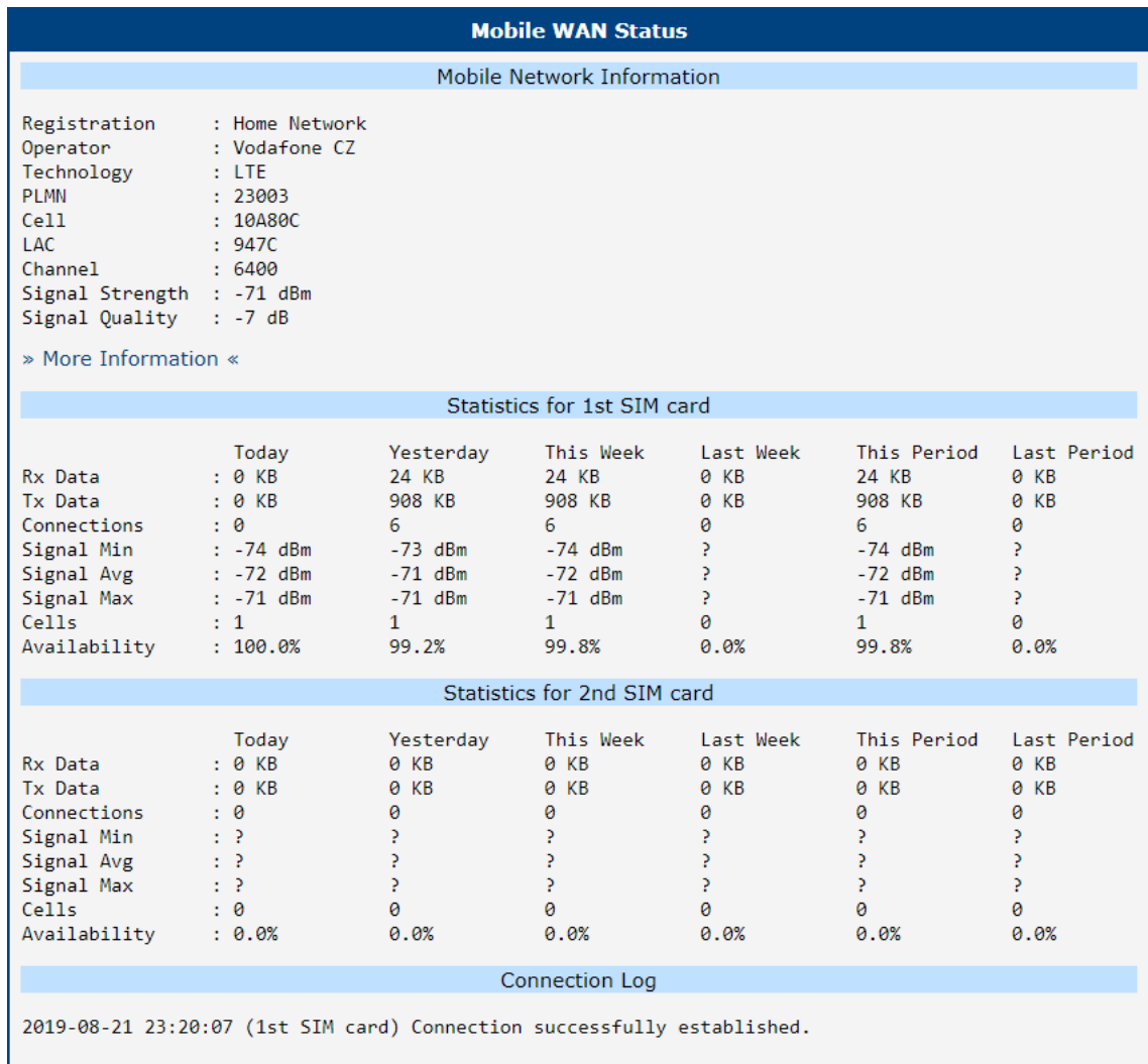
Figure 2: Mobile WAN status
