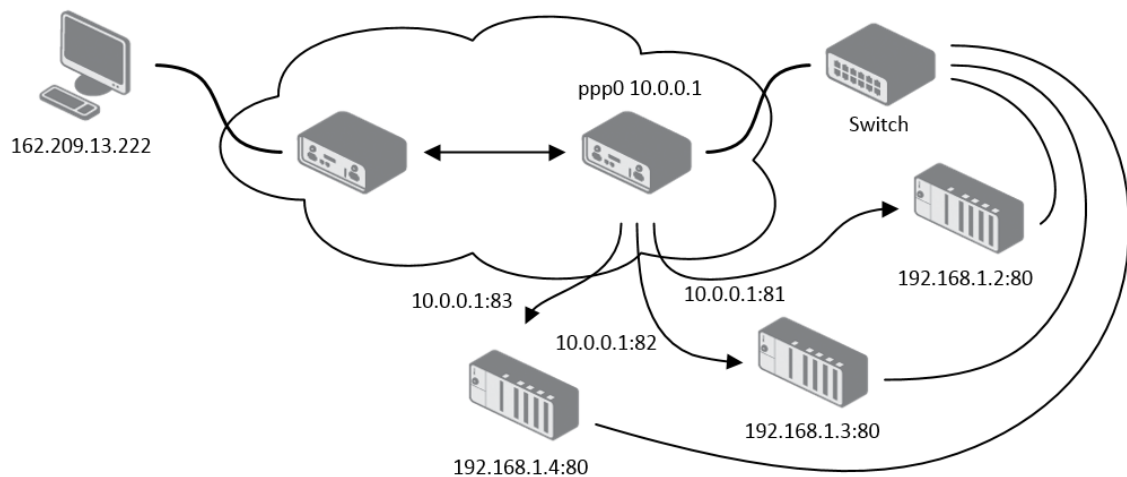
Figure 29: Example 2 – Topology of NAT Configuration
