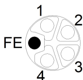
Figure 8: Schematic diagram of the M12 L-coding (socket X04 for Power Out)
