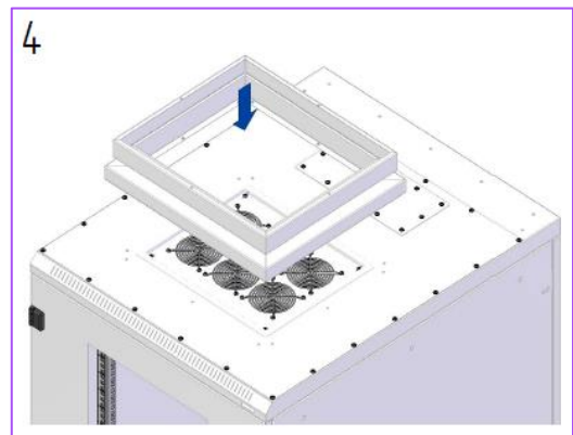
4 Mount cover holder of EDAI200x on adapter (Use enclosed sealer tape on top and bottom)
