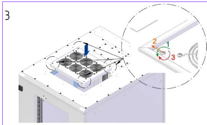
3 Install Fan unit in adapter's cutout.
