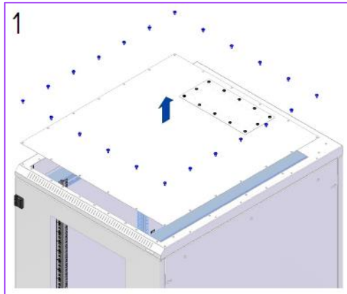
1 Remove top panel from EDI Cabinet
