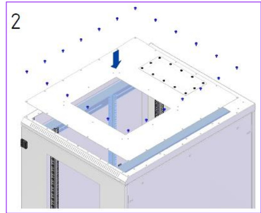
2 Install adapter of EDAI1xxx on cabinet. Adapter size should match cabinet's width / depth
